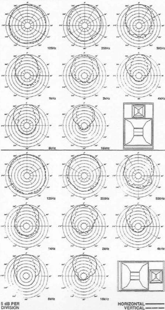
FIGURE 3 — Polar Response
